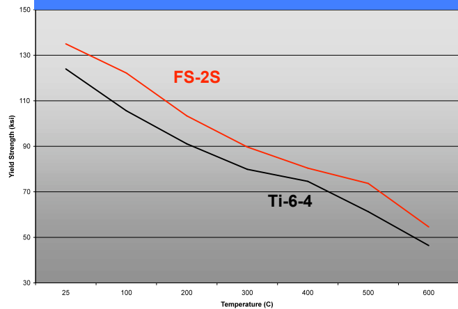
Elevated Temperature Properties of FS-2S vs Ti-6-4 Castings
