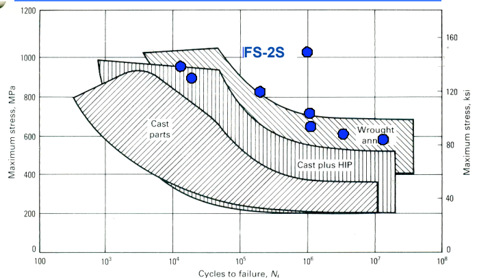
Smooth Bar Axial Fatigue Behavior of FS-2S vs. Ti-6-4 (R=+0.1) FS-2S HIP'd & Stress Relief Annealed
